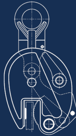
Universal Plate Clamp
